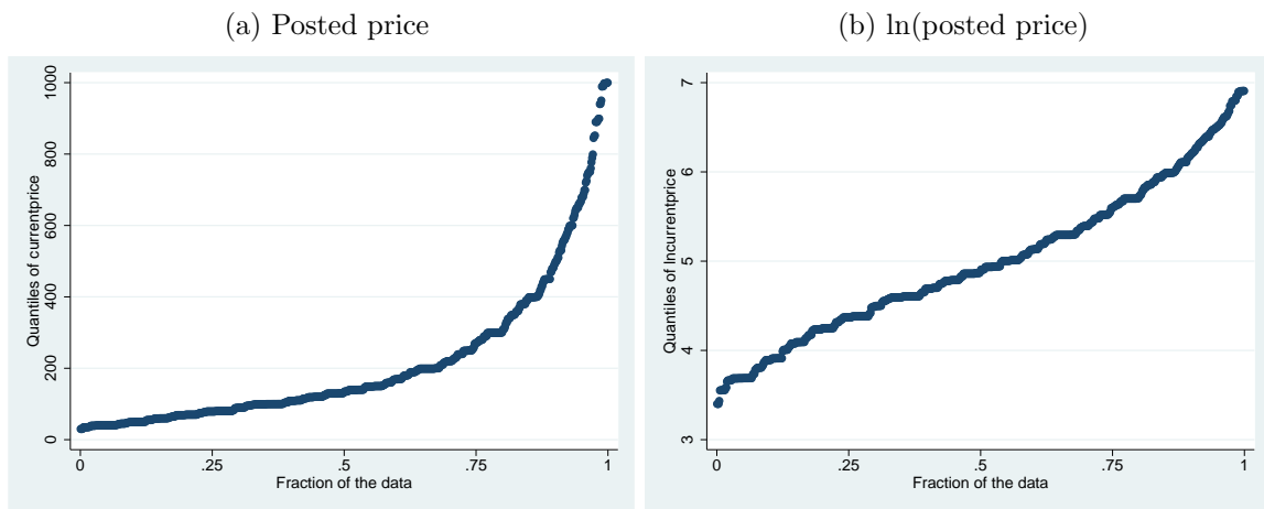
Figure 4: Quantile plots
