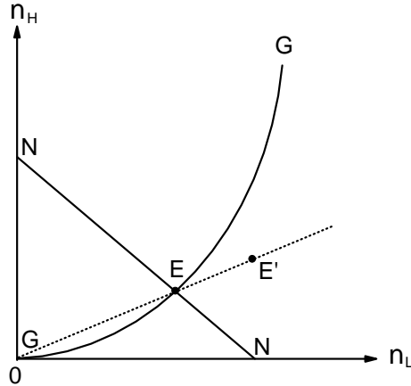
Figure 1: Autarky equilibrium
